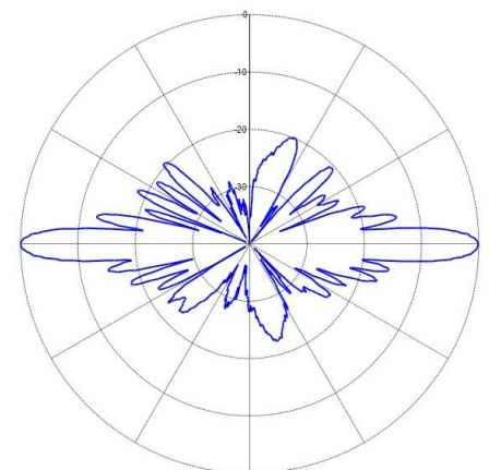
Vertical, 0° downtilt
